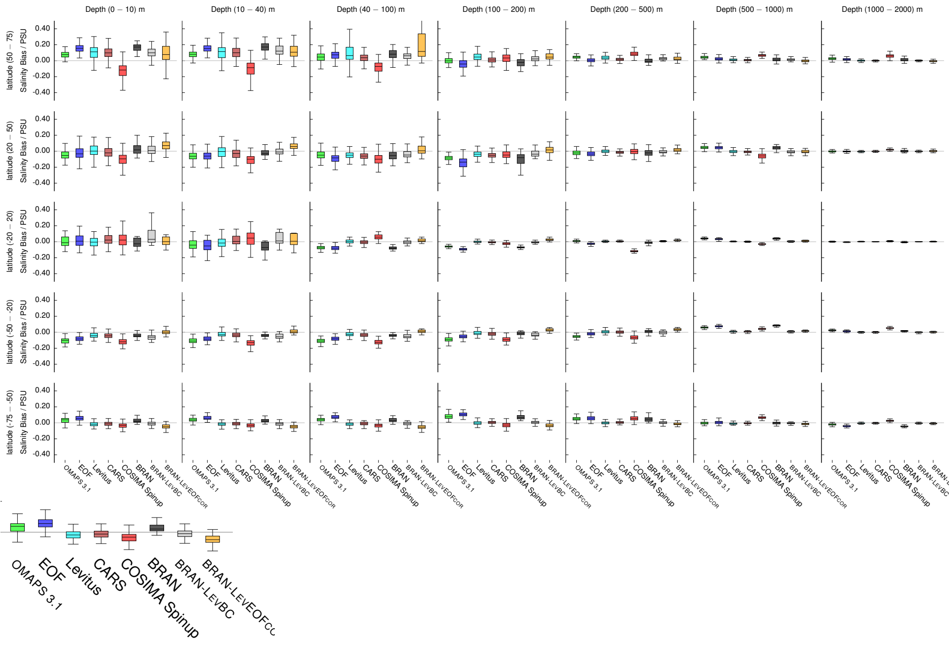
Salinity Bias compared to observations (2016) (5/Jul-Dec)
