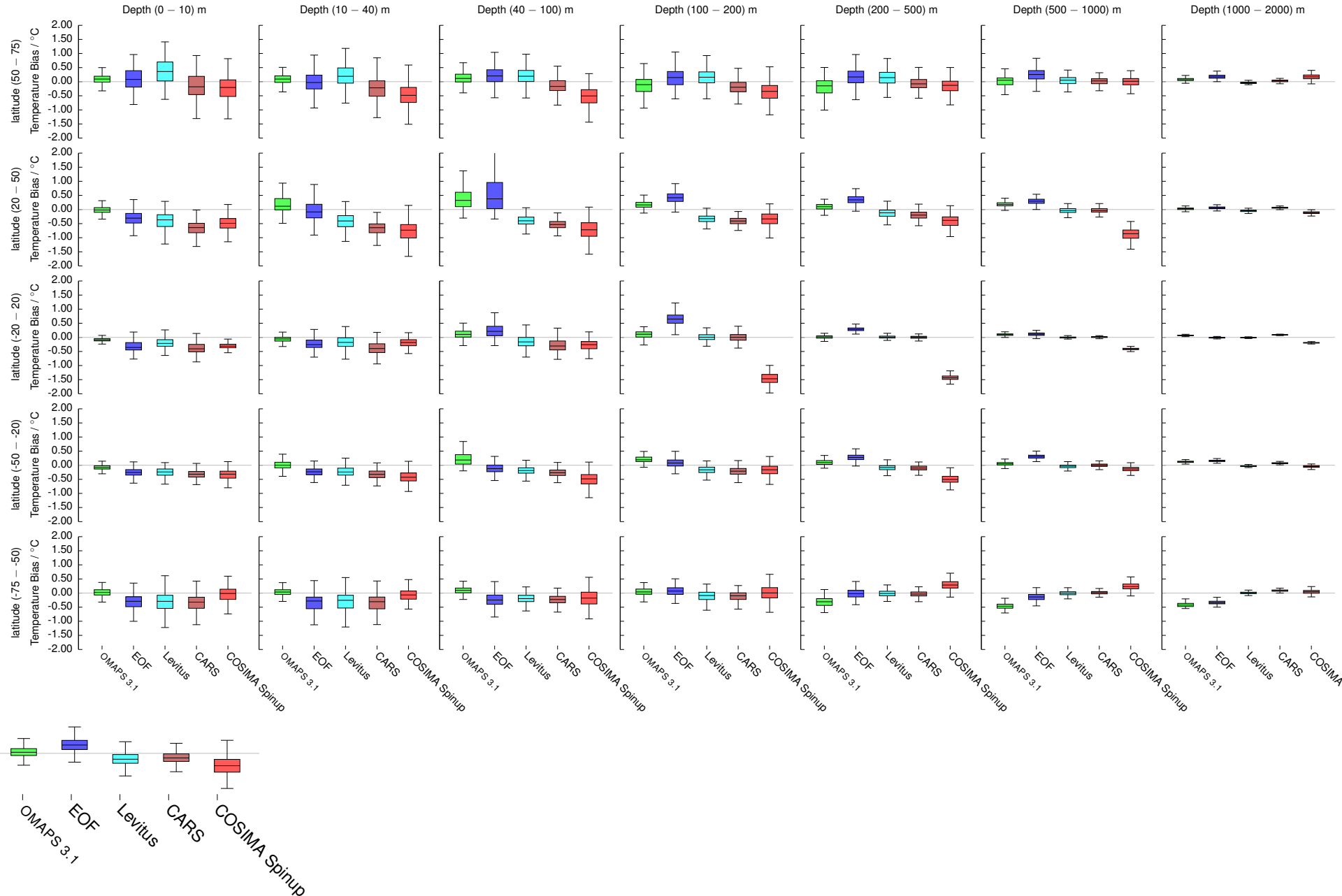
Temperature Bias compared to observations (2017)
