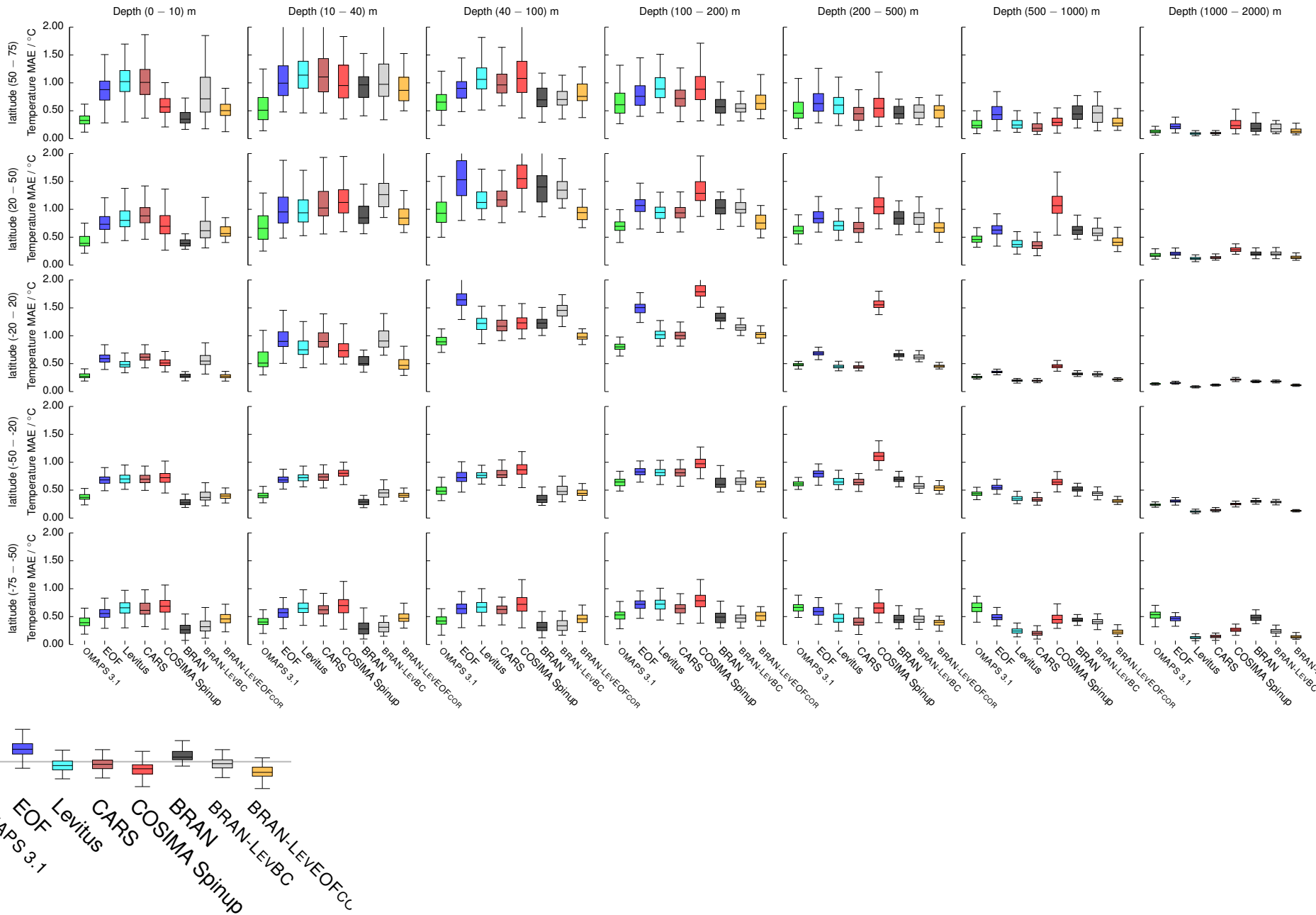
Temperature Mean Absolute Error compared to observations (2016) (5/Jul-Dec)
