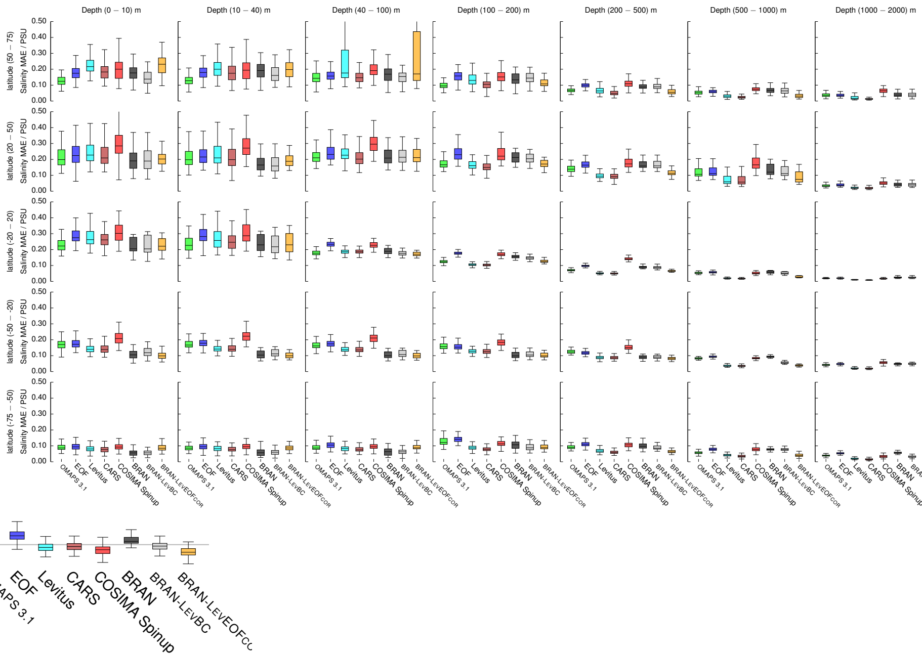
Salinity Mean Absolute Error compared to observations (2016) (5Jul-Dec)
